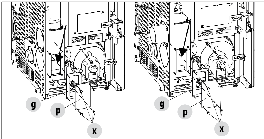
CLEANING THE UPPER SMOKE OUTLET
